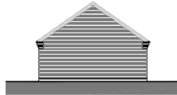
03 SIDE ELEVATION 1/50
