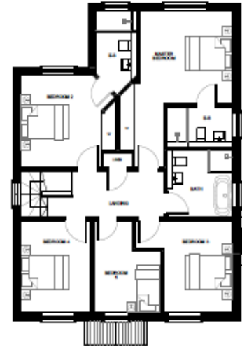
02 FIRST FLOOR PLAN 1:50
