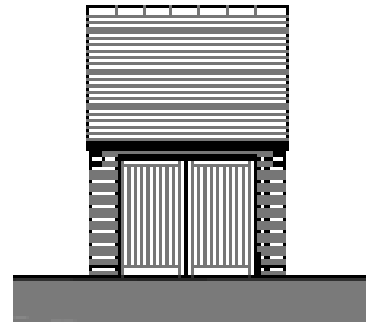
02 FRONT ELEVATION 1/50
